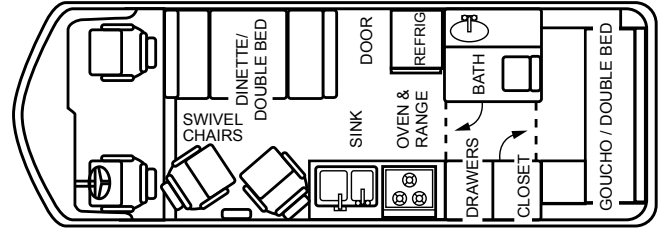
FLOOR PLAN 26'-8
