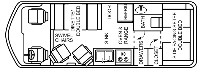
FLOOR PLAN 26'-9
