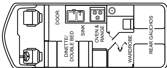
FLOOR PLAN 23'-5
